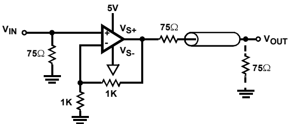
FIGURE 28. SYNC PULSE REMOVER
