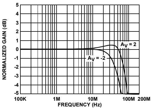
FIGURE 34. VIDEO LINE DRIVER FREQUENCY RESPONSE
