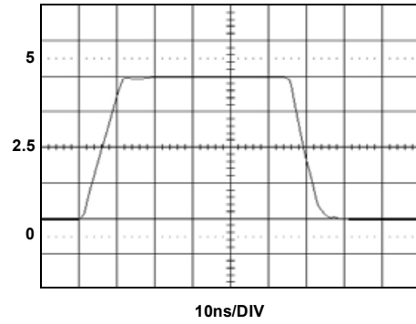
FIGURE 20. LARGE SIGNAL TRANSIENT RESPONSE
