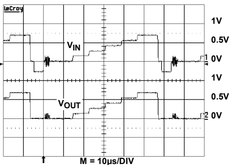
FIGURE 29. VIDEO SIGNAL
