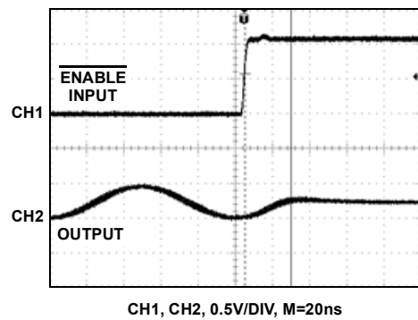
FIGURE 24. DISABLED RESPONSE
