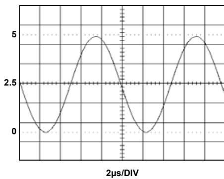
FIGURE 23. OUTPUT SWING
