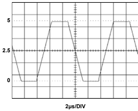
FIGURE 21. OUTPUT SWING
