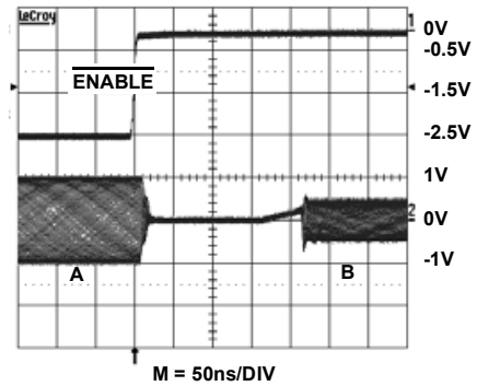
FIGURE 31. ENABLE SIGNAL
