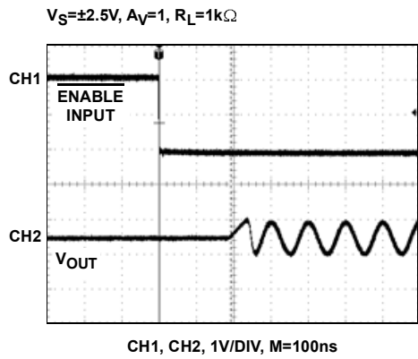
FIGURE 25. ENABLED RESPONSE
