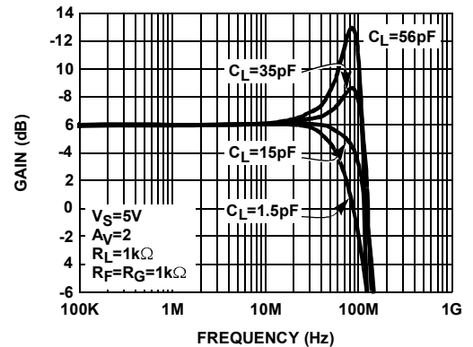
FIGURE 6. SMALL SIGNAL FREQUENCY RESPONSE FOR VARIOUS C_L
