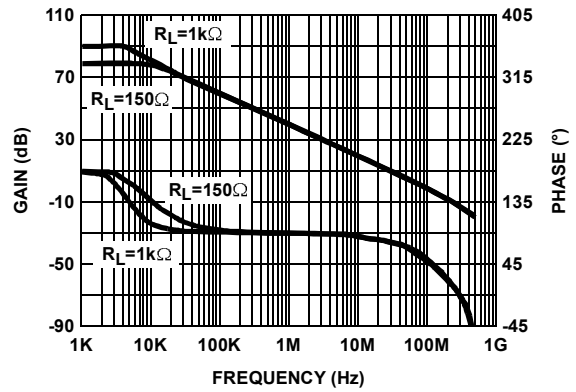
FIGURE 8. OPEN LOOP GAIN AND PHASE vs FREQUENCY
