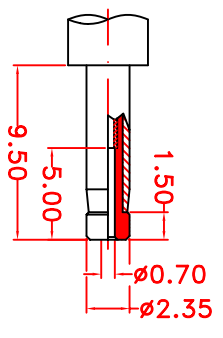
MATE PLUG
