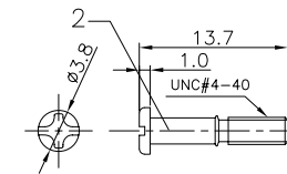
Short BOLT
